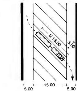
① 45° parking, truck with trailer
